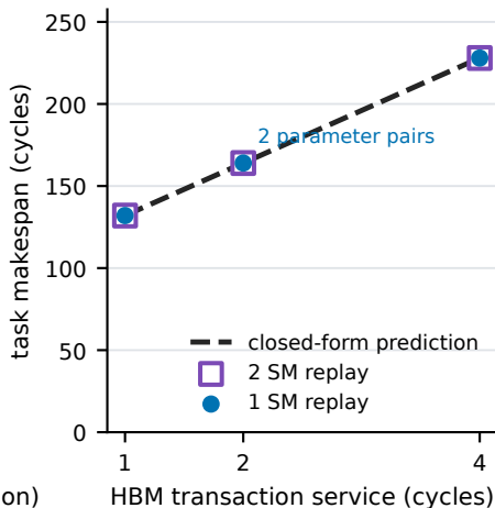
(b) Memory-bound
