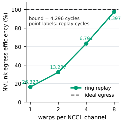
(c) Network-bound
