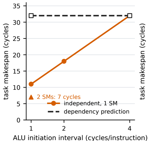
(a) Compute-bound
