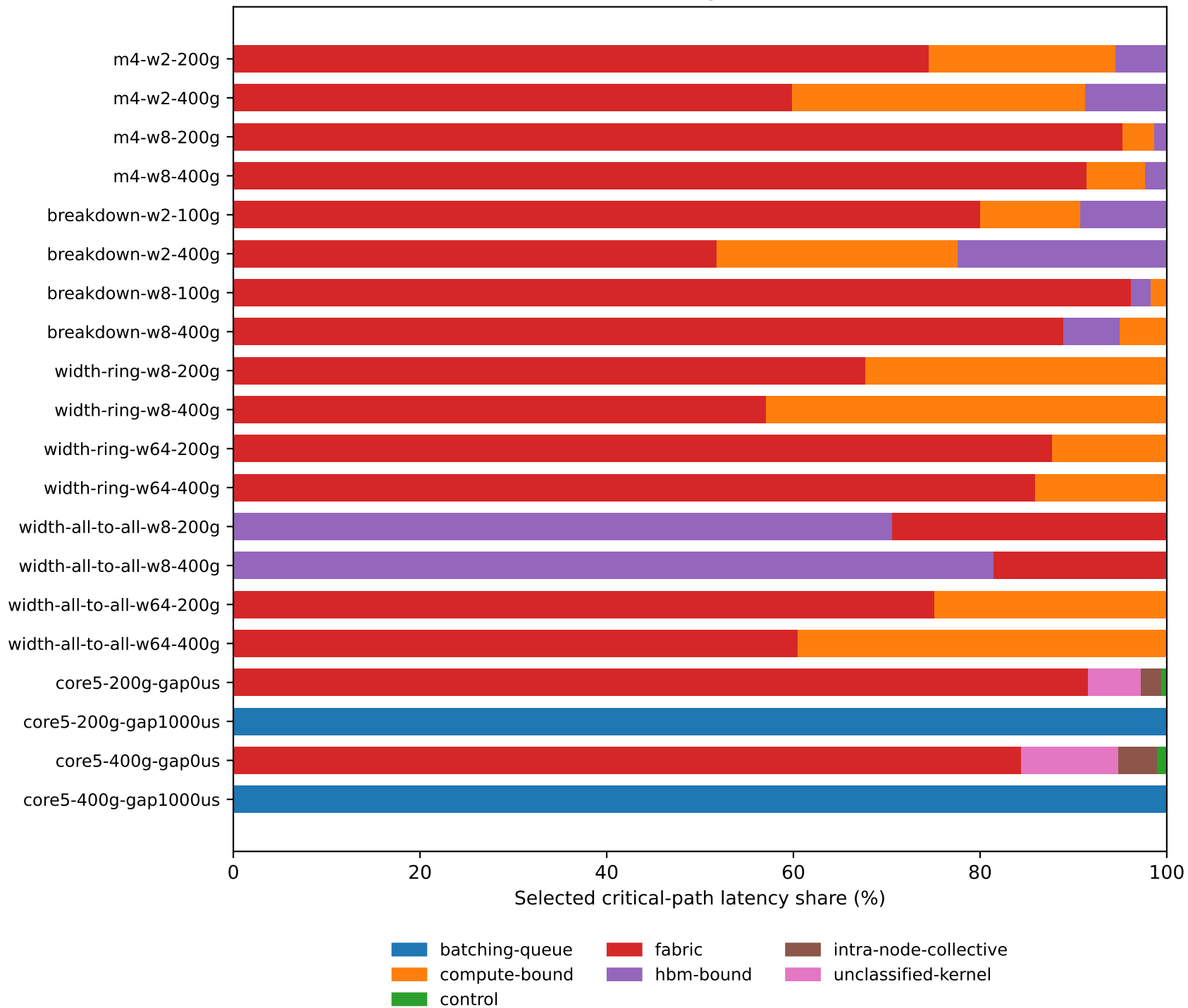
Bottleneck classes, largest contribution first
