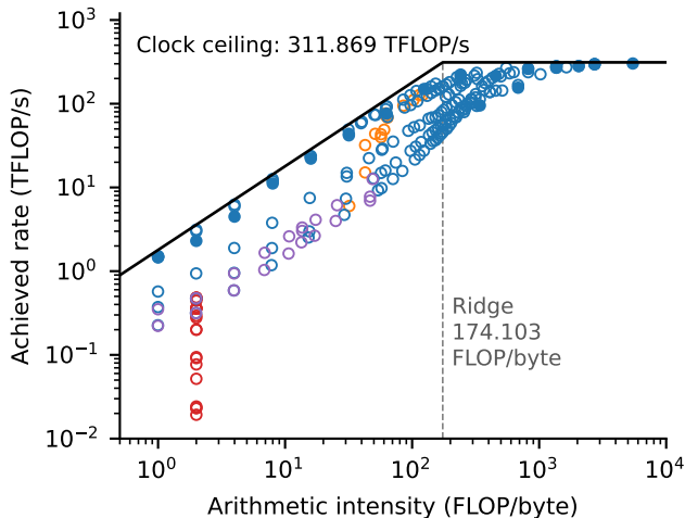
A: A100 arithmetic roofline
