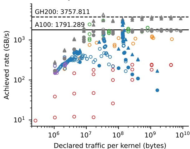
B: Memory rates, both devices
