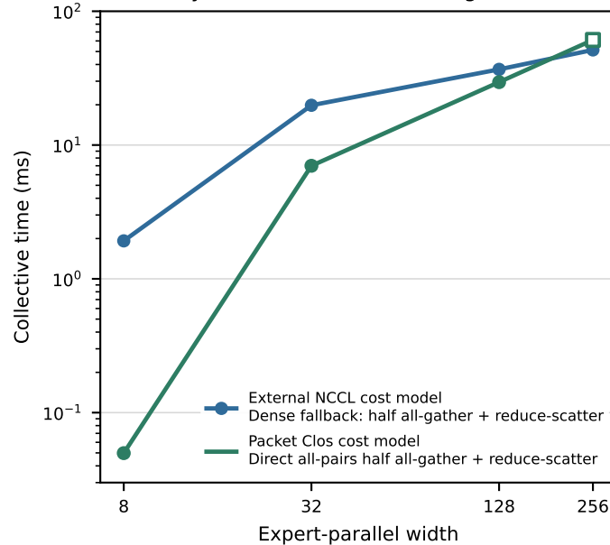
Family D cost models, same logical count
