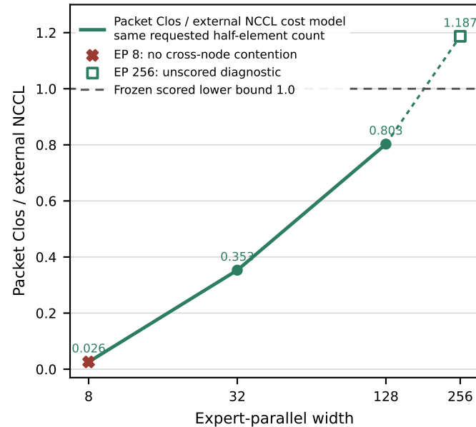
Family D cost-model ratio
