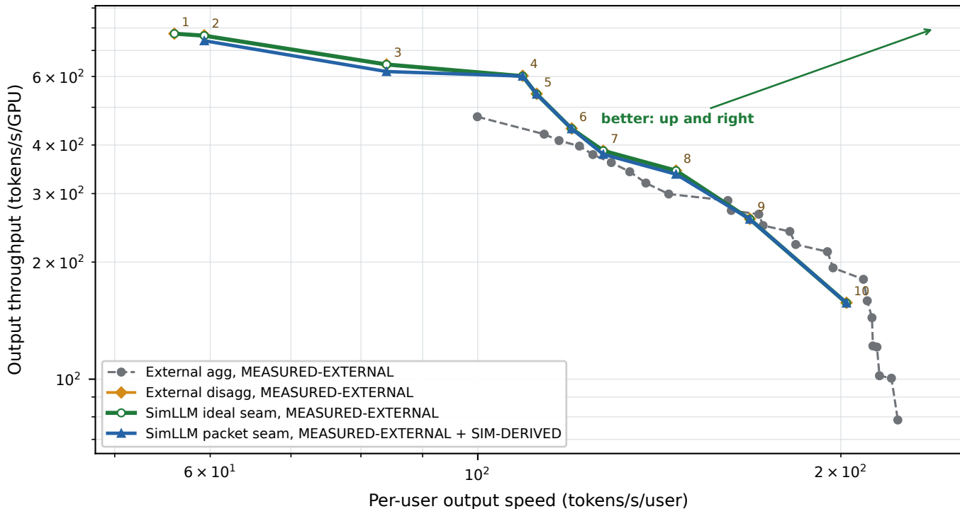
Qwen3-32B FP8 matched-seam deployment frontier
