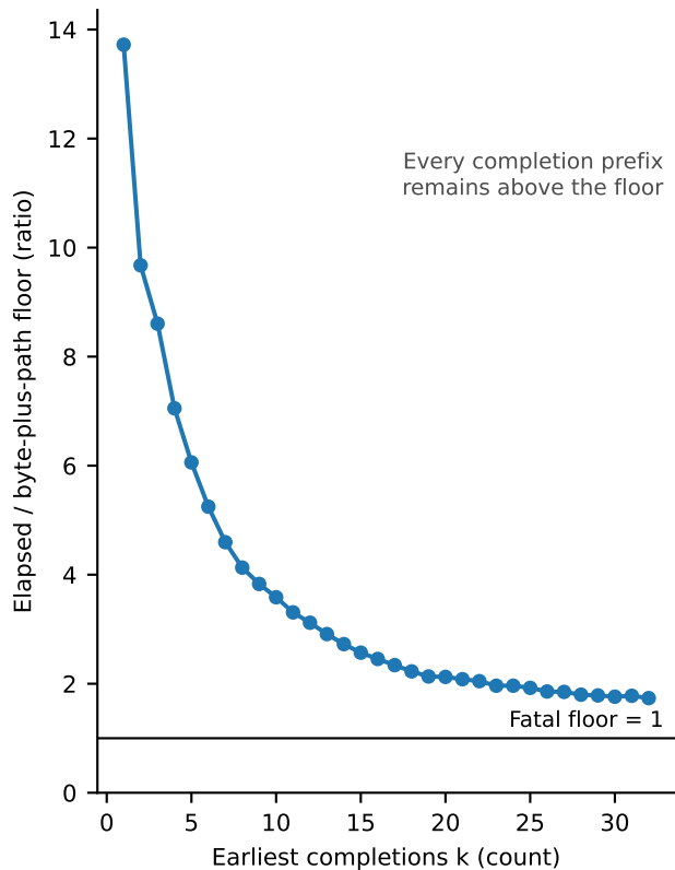
(b) Completion-prefix floor 32 senders, 64 KiB, 200 Gbit/s
