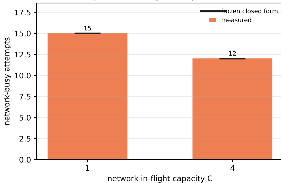
Backpressure: busy attempts are N - C
