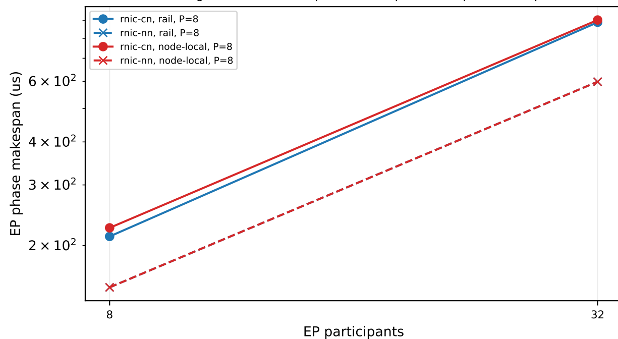
D: background EP all-to-all phase makespan, 1 MiB per remote pair
