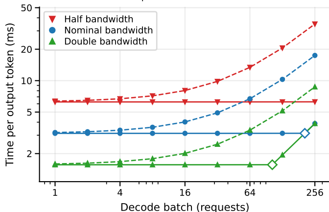
(b) 7B-class dense, TP1 H200 bandwidth sweep
