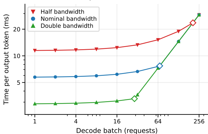
(f) DeepSeek-V3, EP72 rank class 0 H200 bandwidth sweep
