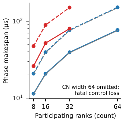
(e) Single-engine expert step Ideal fabric share
