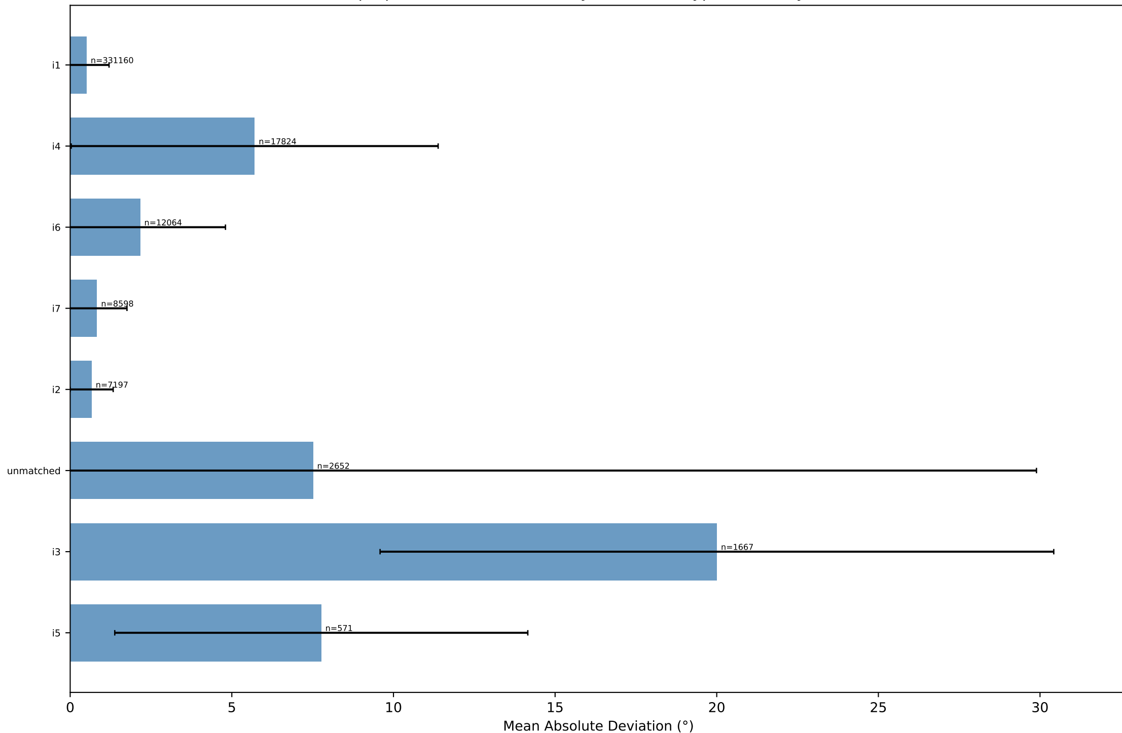
Improper Torsion Deviations by Parameter Type Sorted by Count
