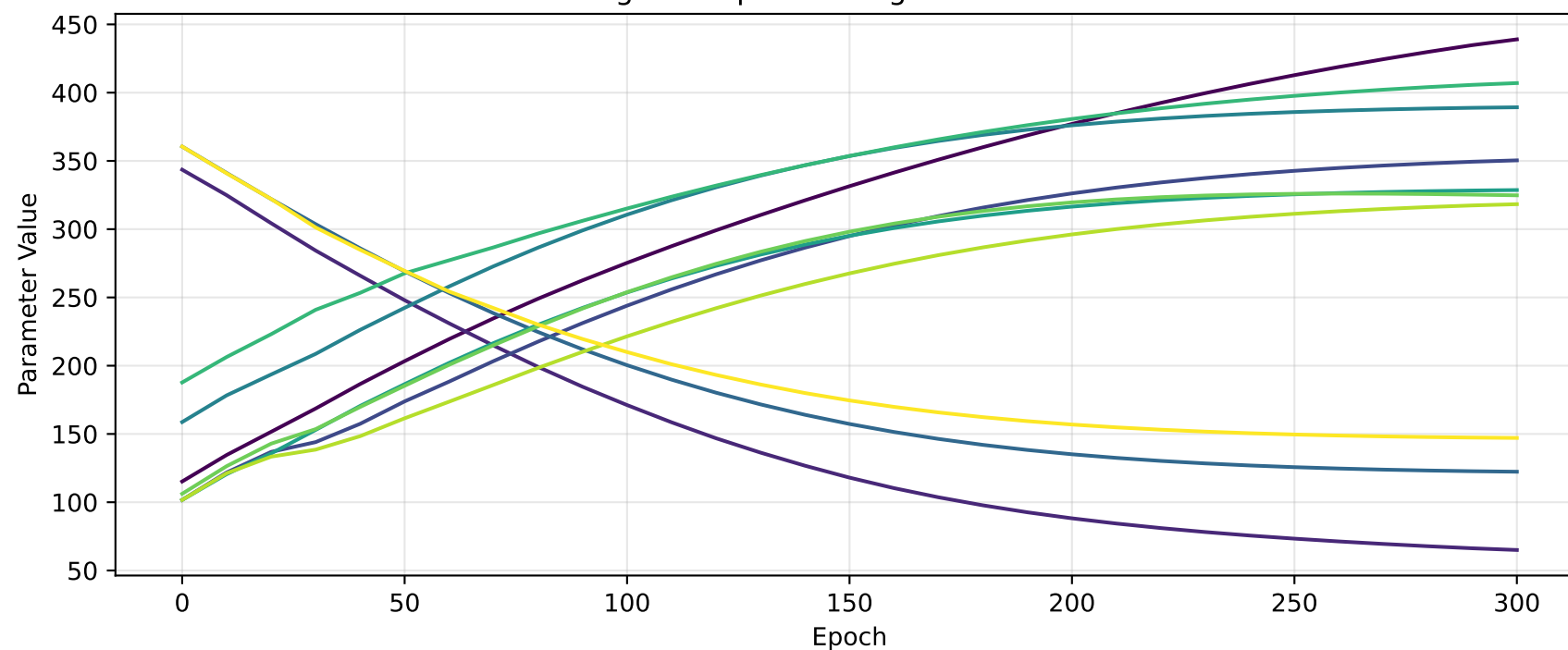
Bonds - Top 10 Changed Parameters
