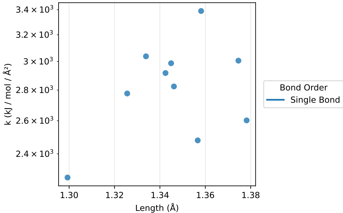
Bonds: k vs length for C-F (10 params)
