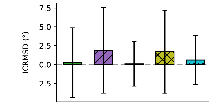
Dihedral RMSD
