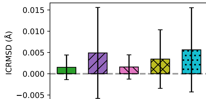
Bond RMSD
