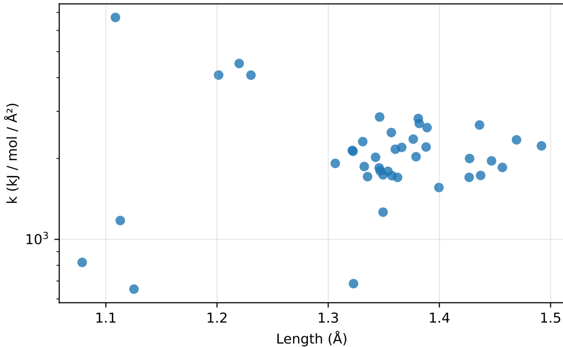
Bonds: k vs length for N-N (41 params)
