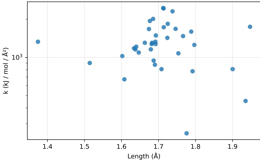
Bonds: k vs length for N-S (37 params)
