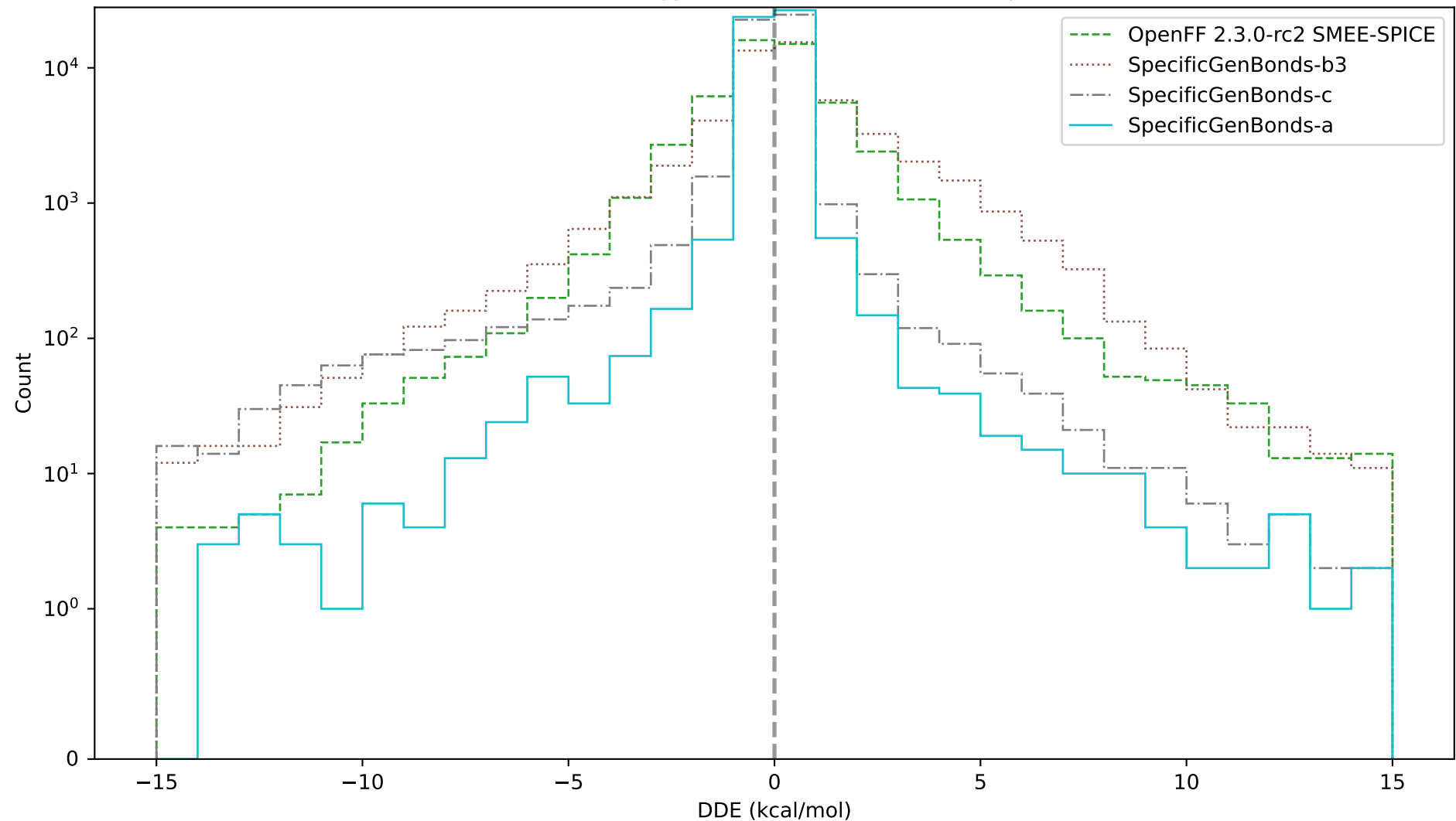
Deformation-Driven Energy Distribution Relative to OpenFF 2.3.0-rc2
