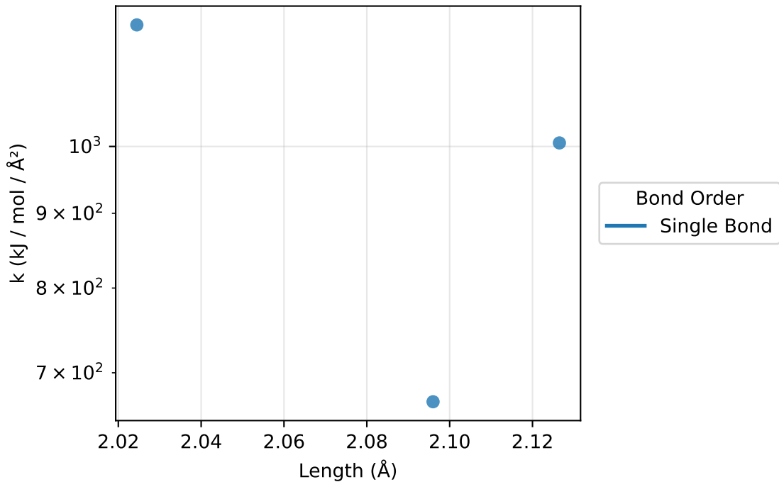
Bonds: k vs length for Cl-S (3 params)
