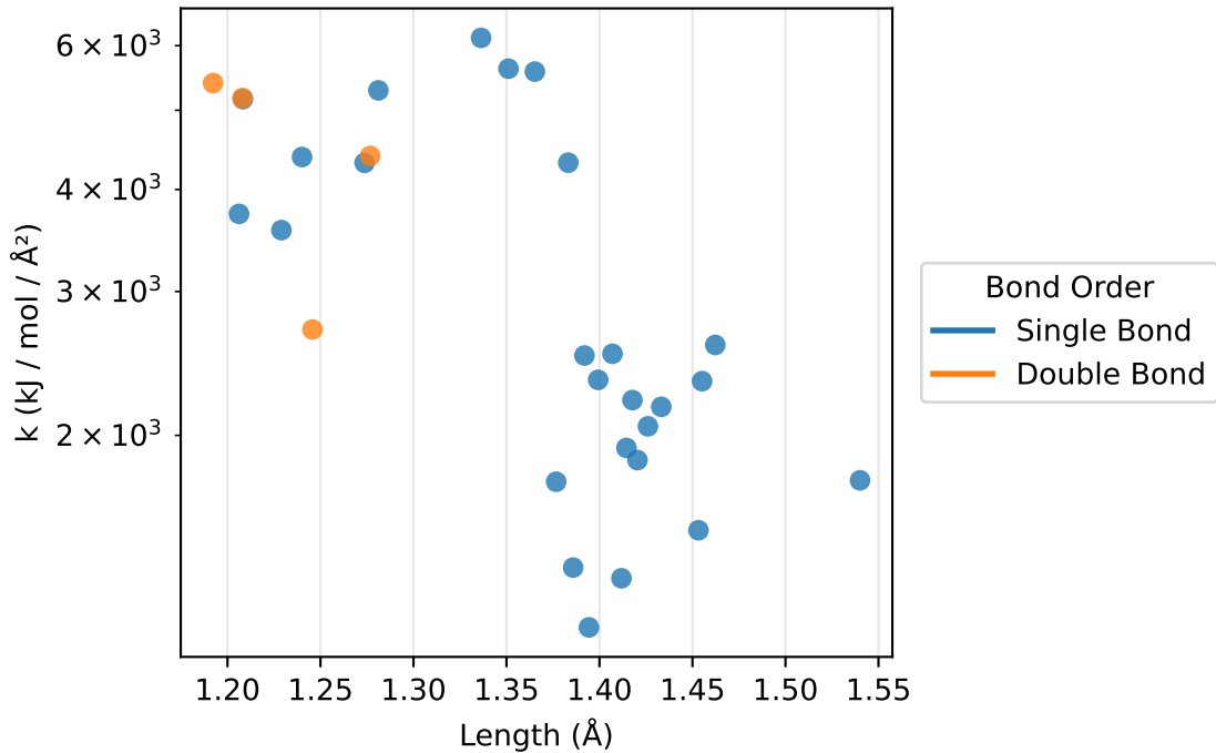
Bonds: k vs length for N-O (30 params)
