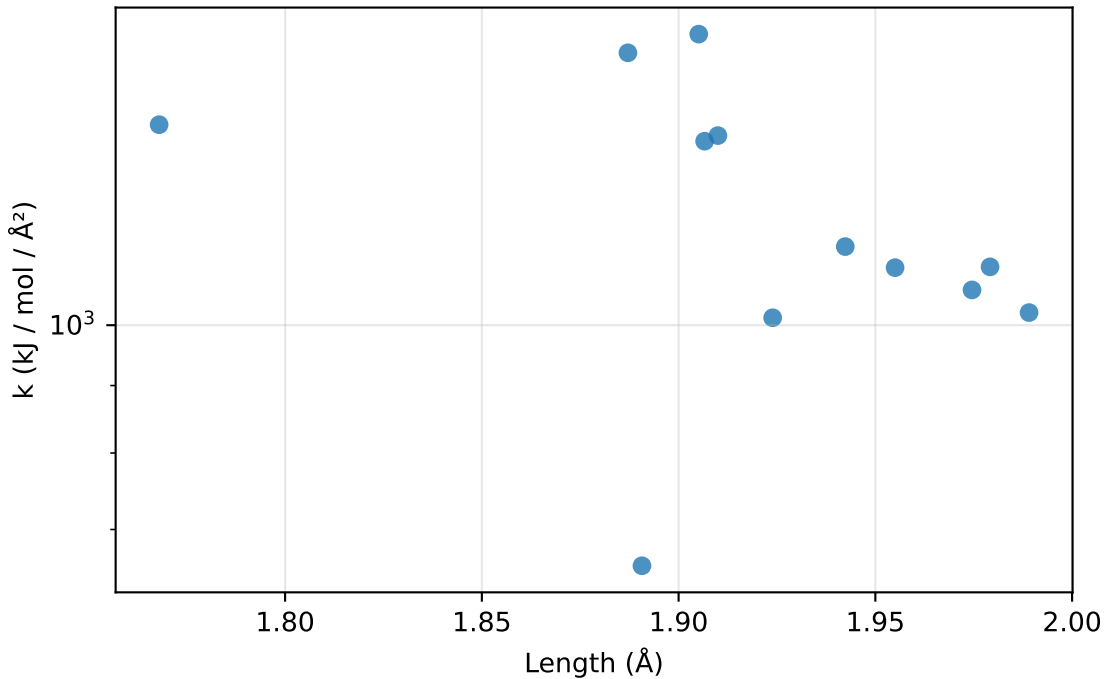
Bonds: k vs length for Br-C (12 params)
