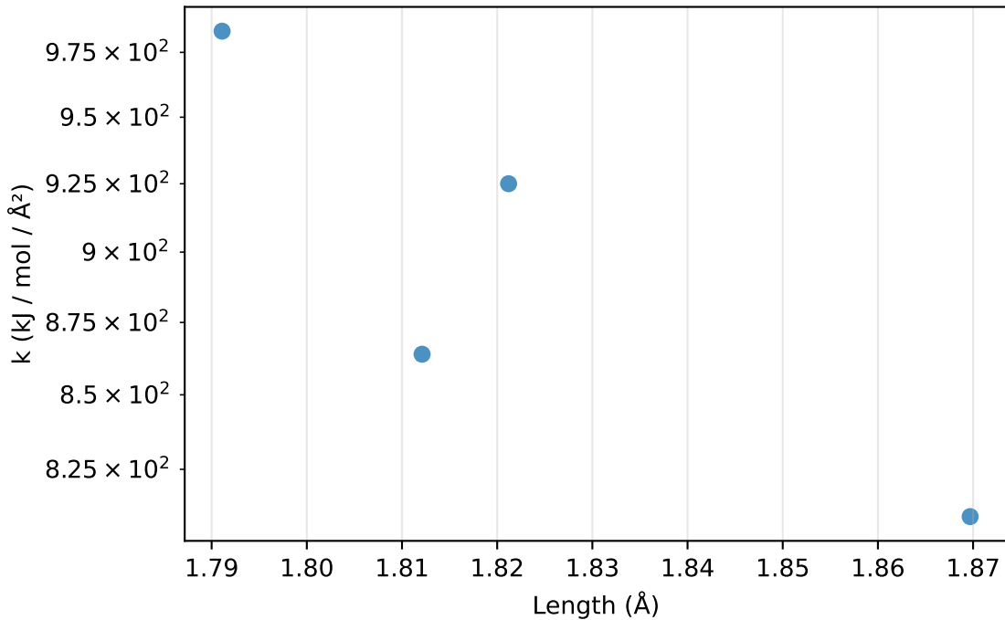
Bonds: k vs length for Br-N (4 params)
