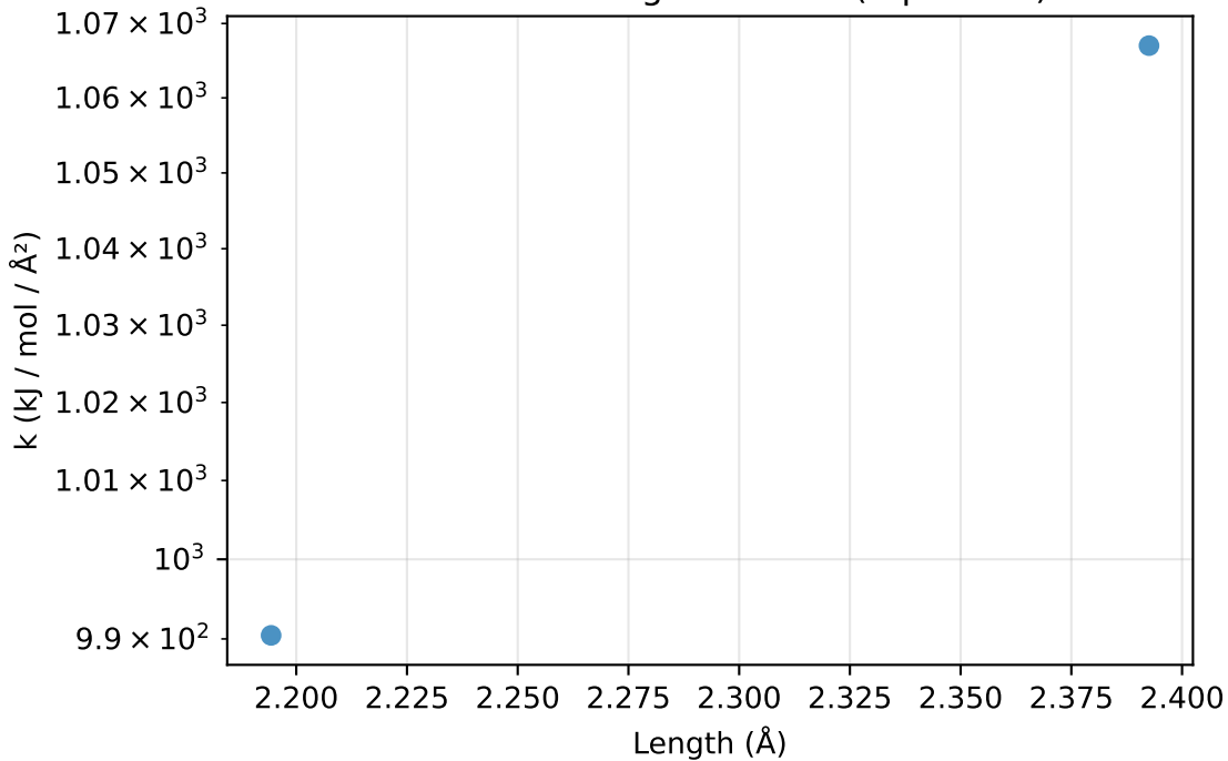
Bonds: k vs length for Br-P (2 params)
