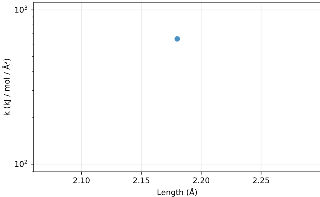
Bonds: k vs length for Br-S (1 params)
