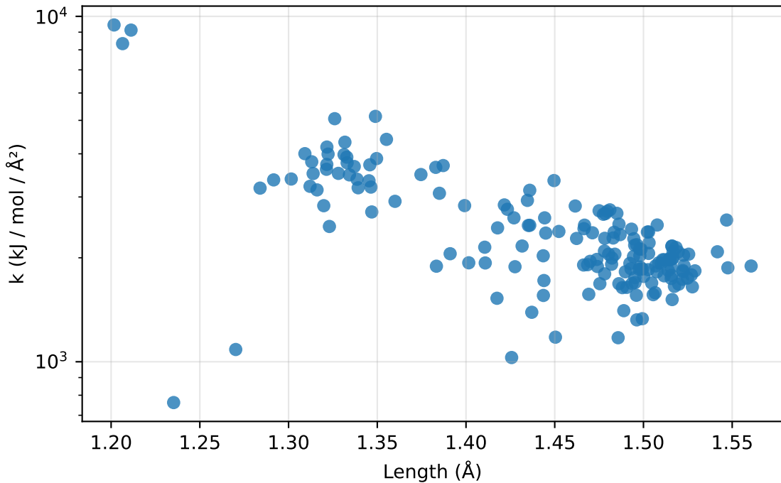
Bonds: k vs length for C-C (171 params)
