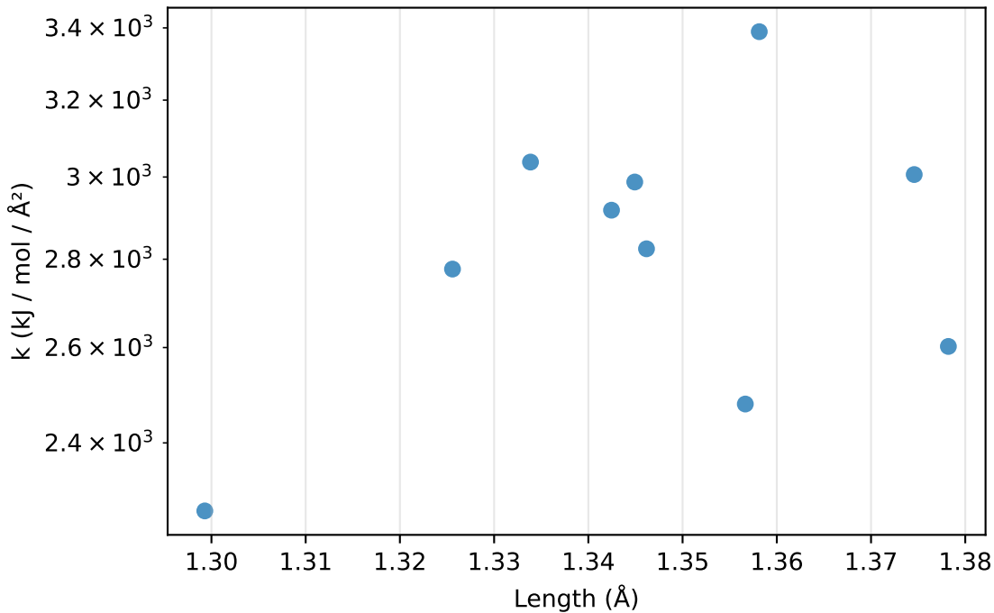
Bonds: k vs length for C-F (10 params)
