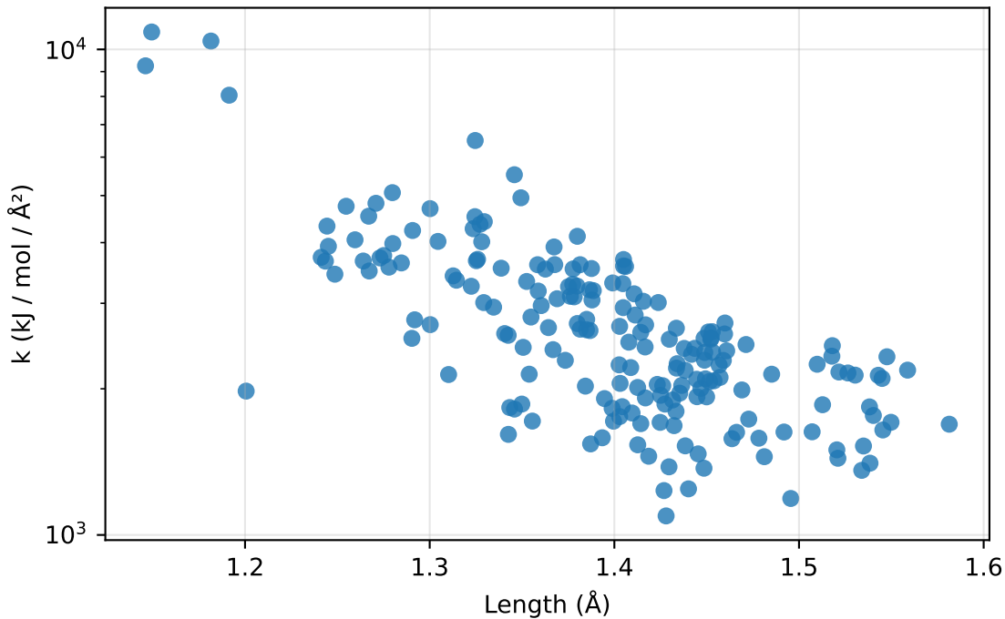
Bonds: k vs length for C-N (193 params)
