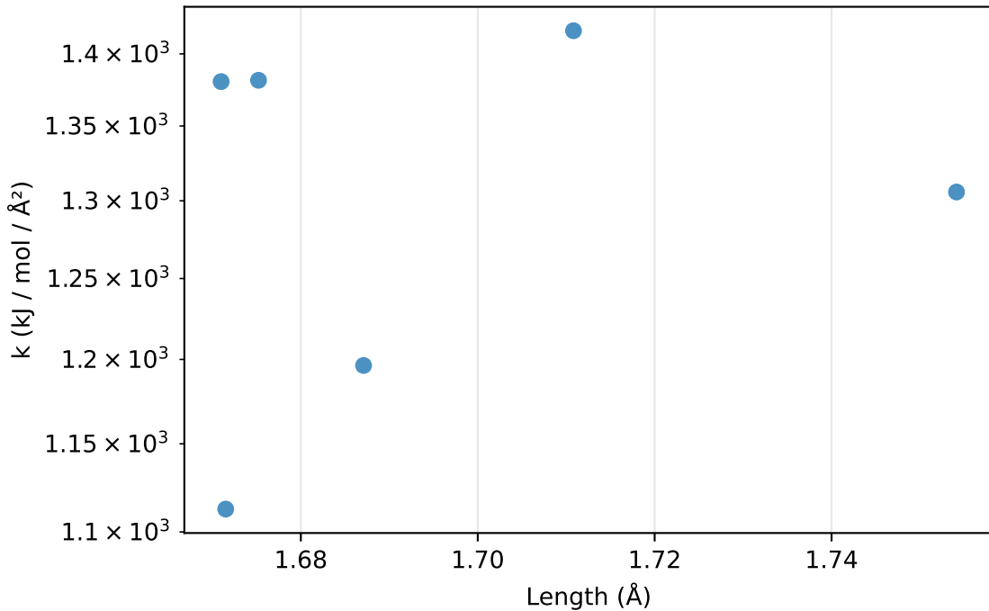
Bonds: k vs length for Cl-N (6 params)
