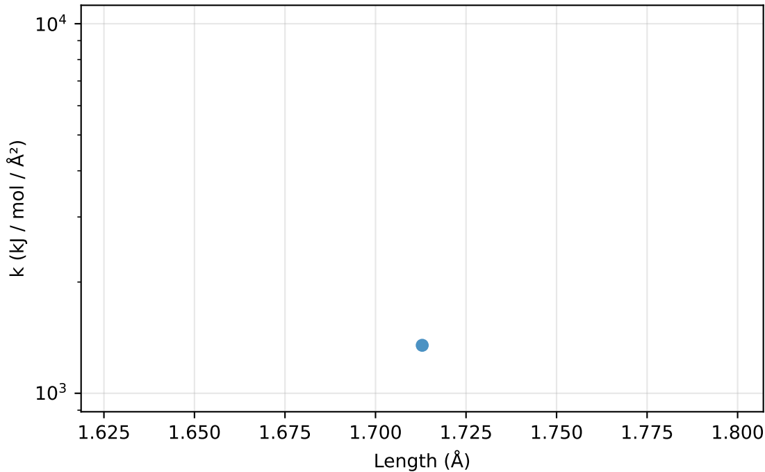
Bonds: k vs length for F-S (1 params)
