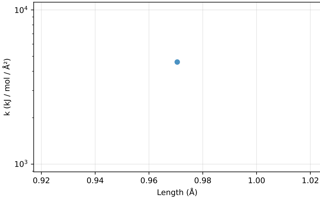
Bonds: k vs length for H-O (1 params)
