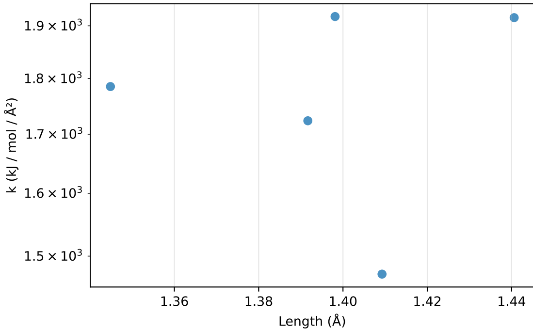
Bonds: k vs length for H-P (5 params)
