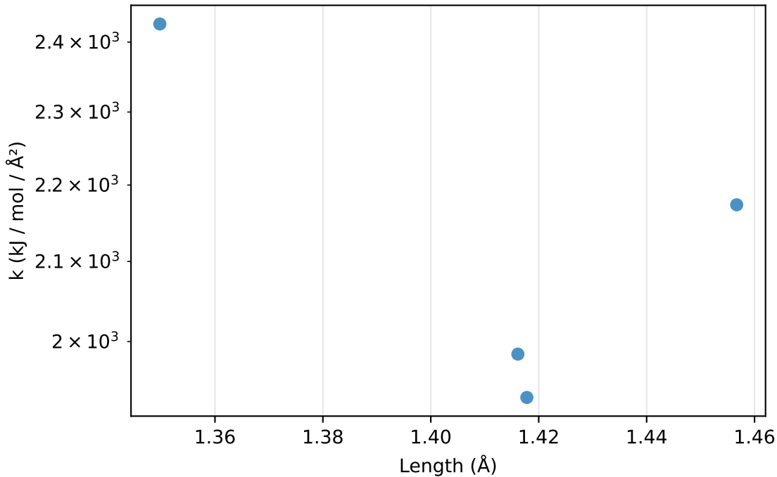
Bonds: k vs length for H-S (4 params)
