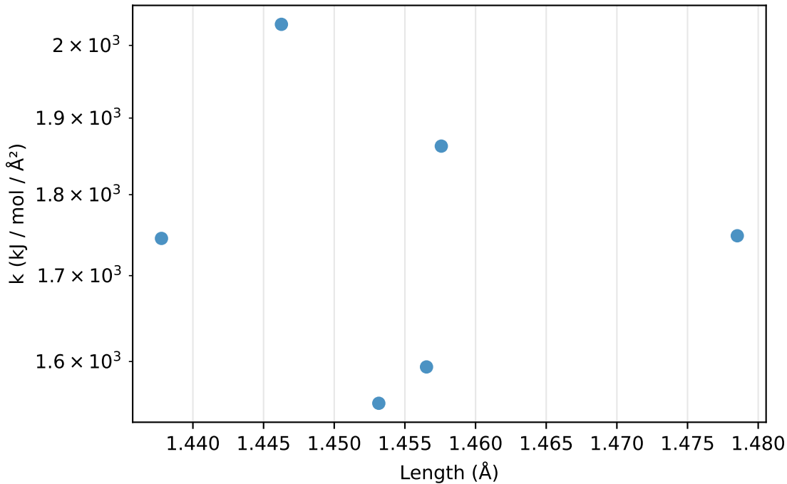
Bonds: k vs length for O-O (6 params)
