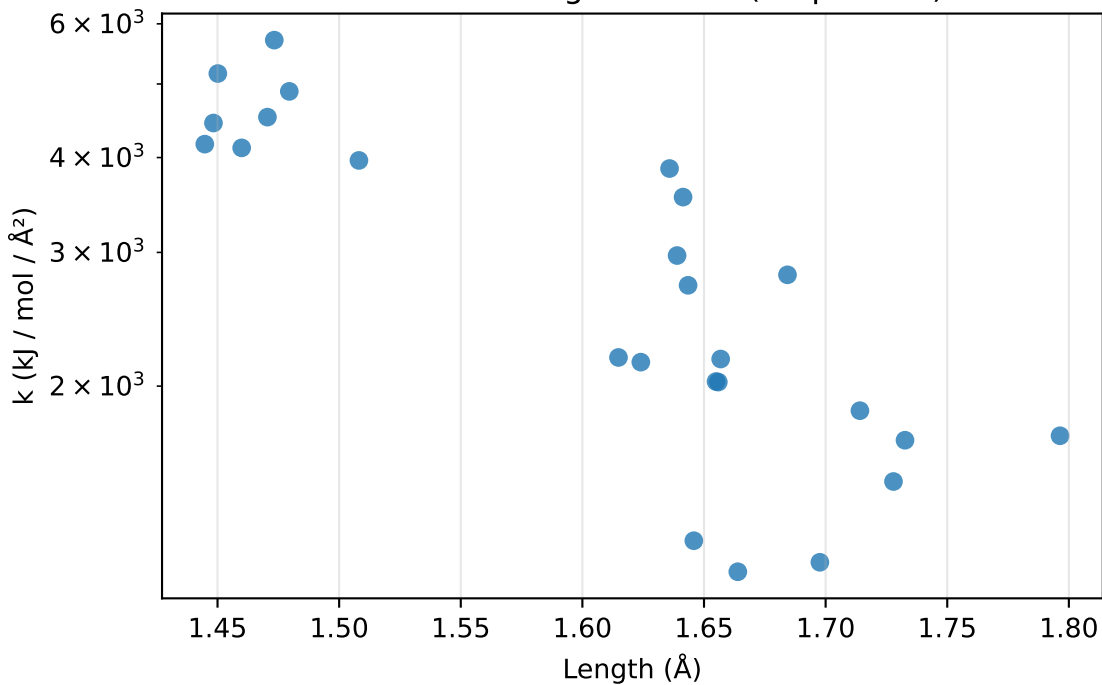
Bonds: k vs length for O-P (25 params)
