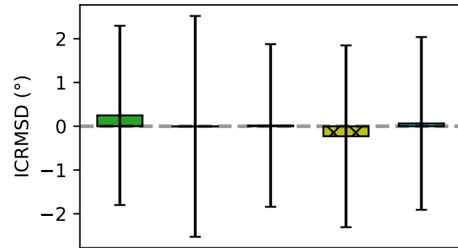
Improper RMSD
