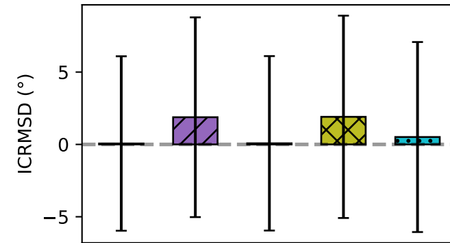
Dihedral RMSD
