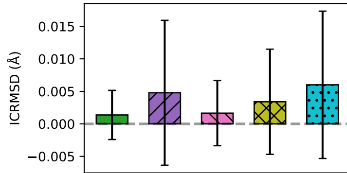
Bond RMSD
