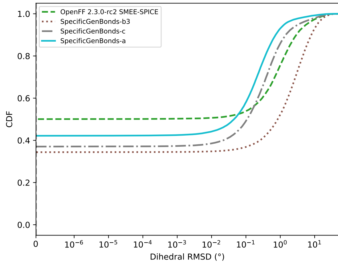
Dihedral Internal Coordinate RMSD
