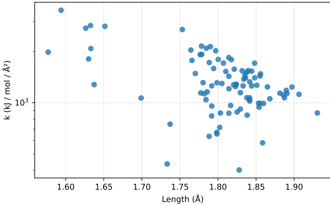
Bonds: k vs length for C-S (91 params)
