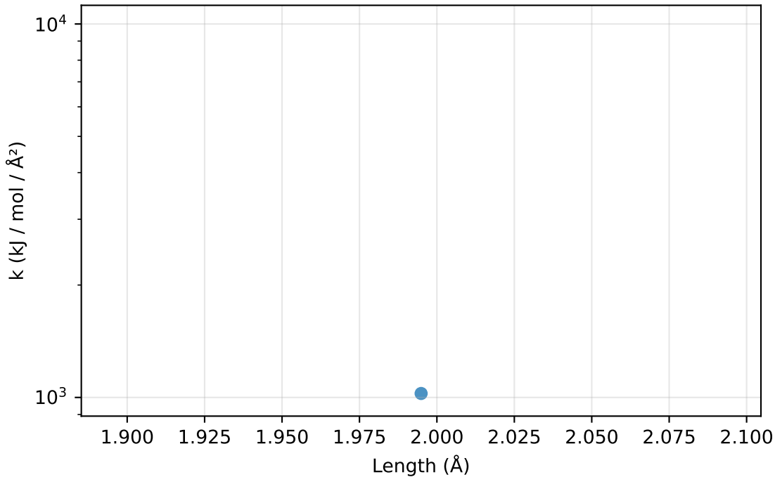
Bonds: k vs length for I-N (1 params)
