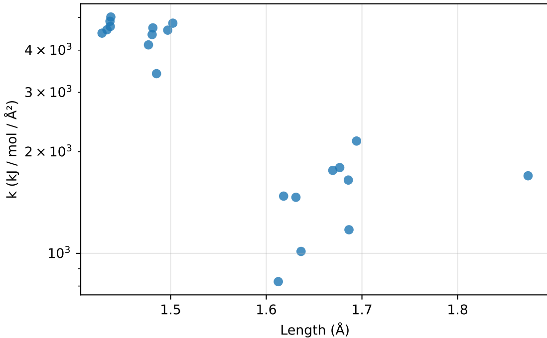
Bonds: k vs length for O-S (21 params)
