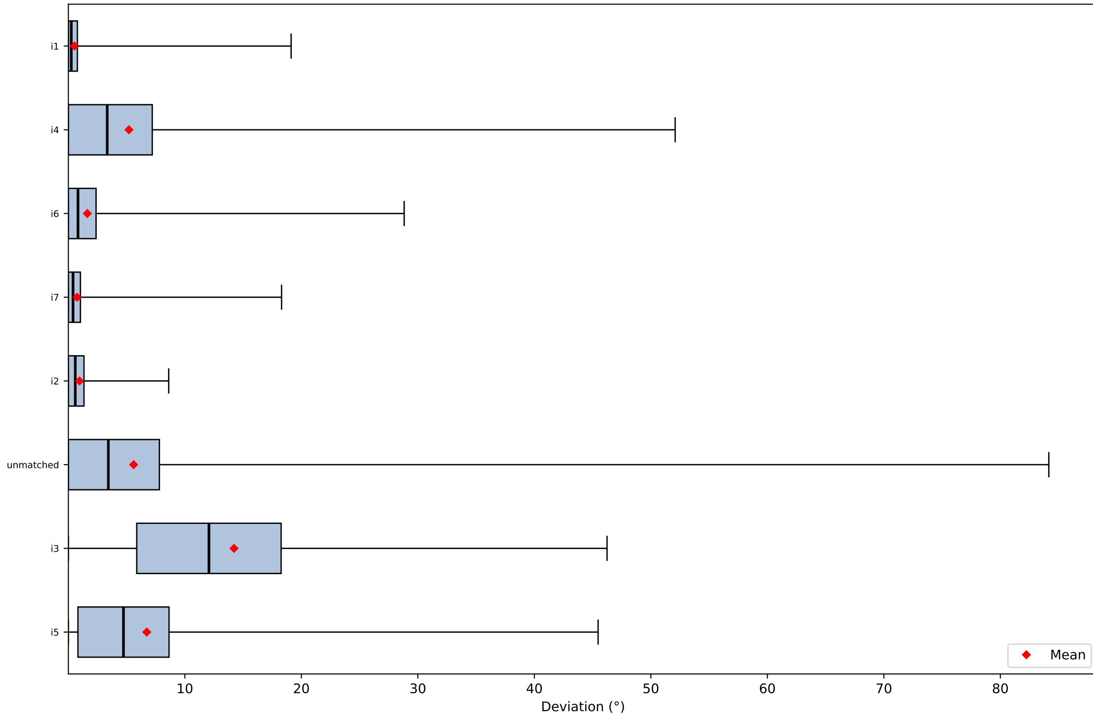
Improper Torsion Deviations Distribution by Parameter Type (All 8 parameters)
