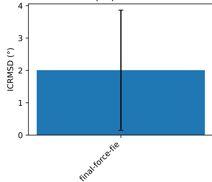
Improper RMSD
