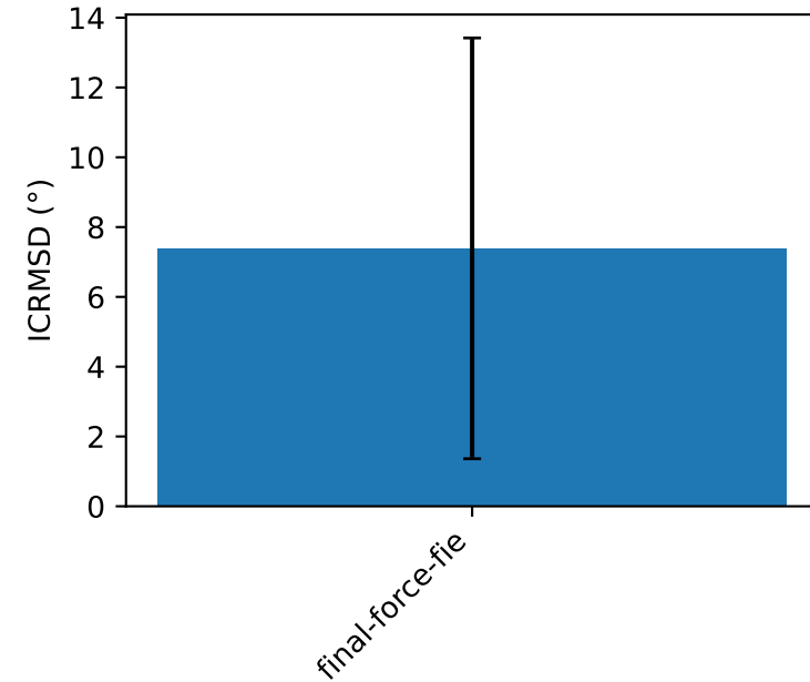
Dihedral RMSD
