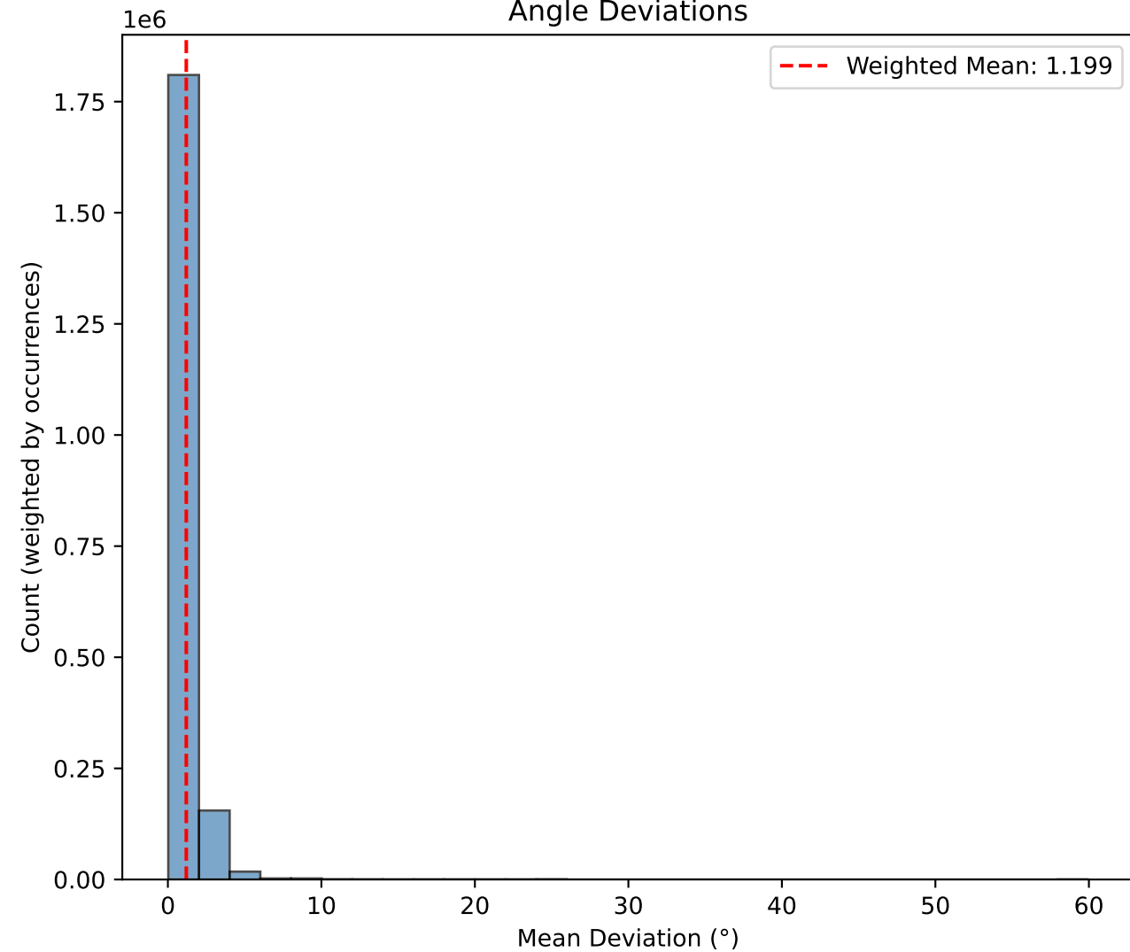
Improper Torsion Deviations
