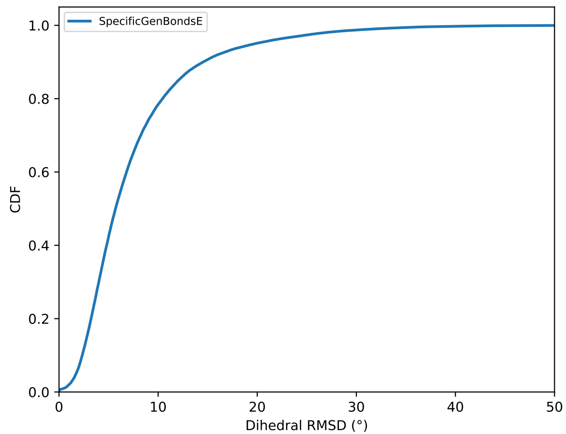
Dihedral Internal Coordinate RMSD
