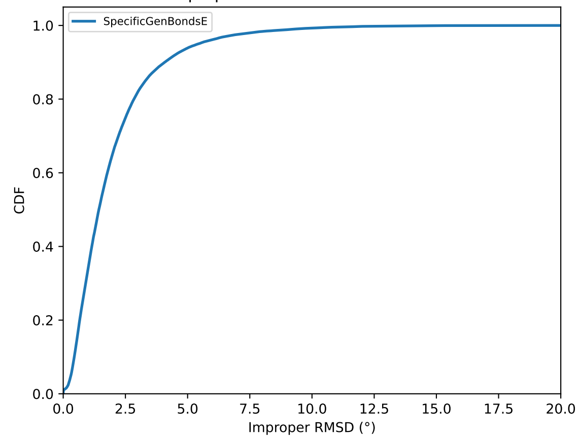
Improper Internal Coordinate RMSD
