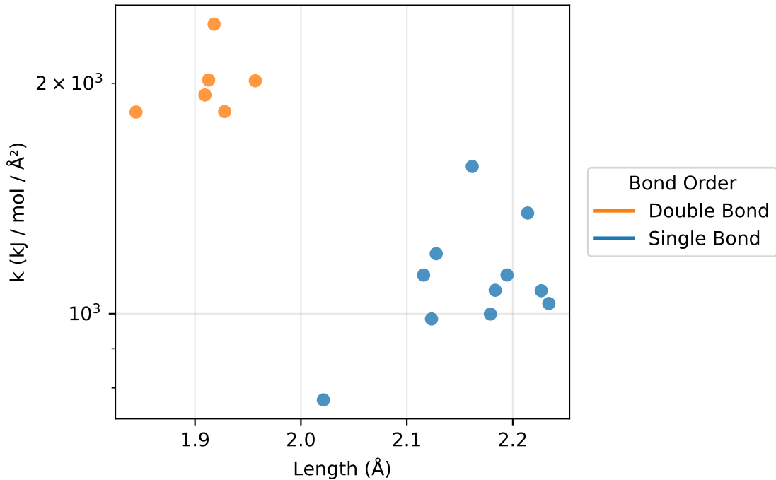
Bonds: k vs length for P-S (17 params)
