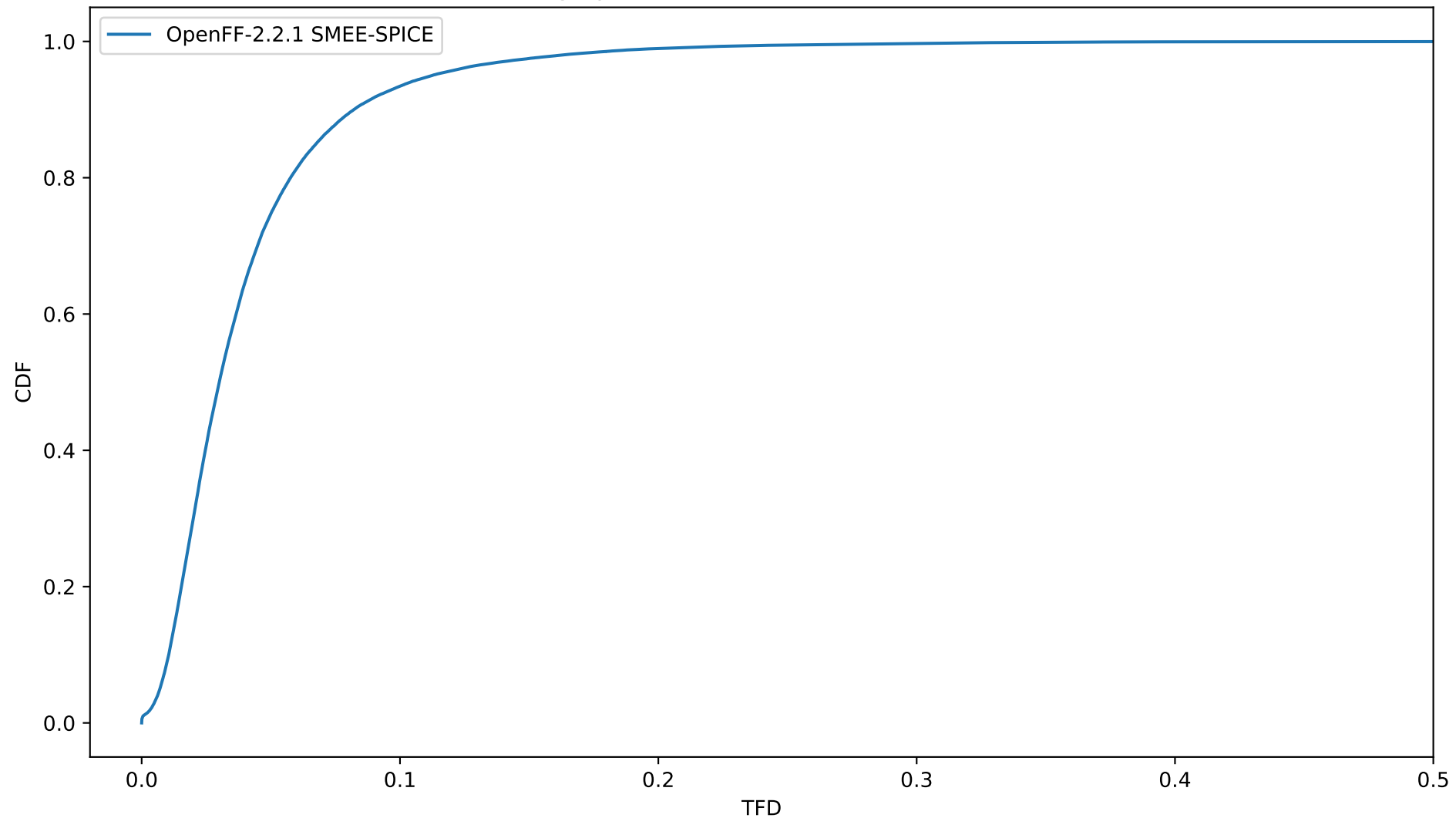
Torsion Fingerprint Deviation - Cumulative Distribution
