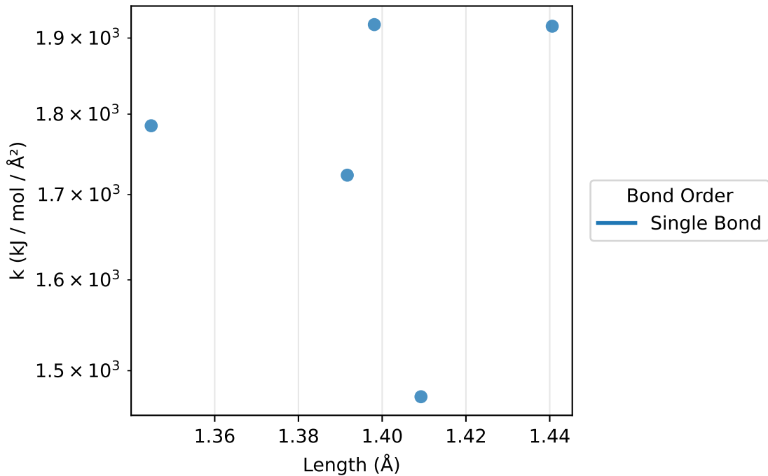
Bonds: k vs length for H-P (5 params)
