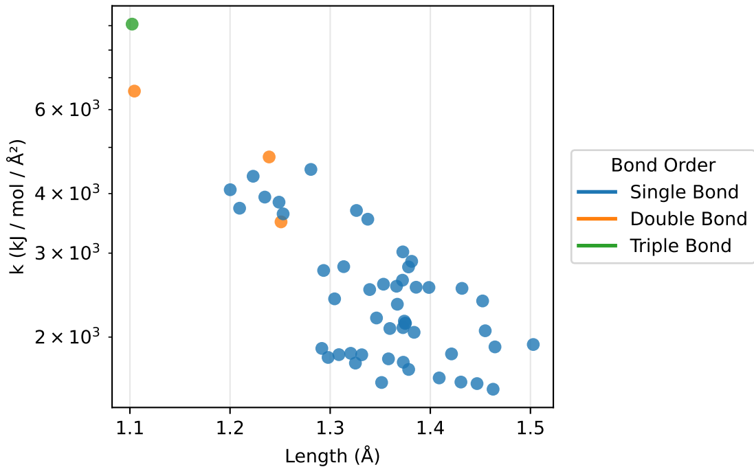
Bonds: k vs length for N-N (53 params)
