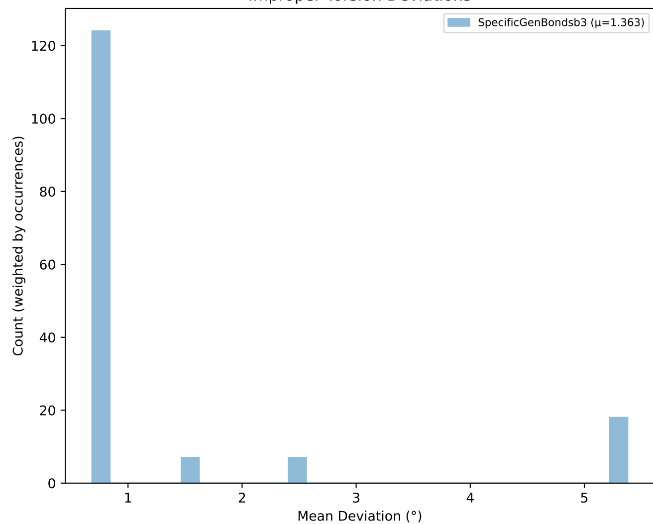
Improper Torsion Deviations
