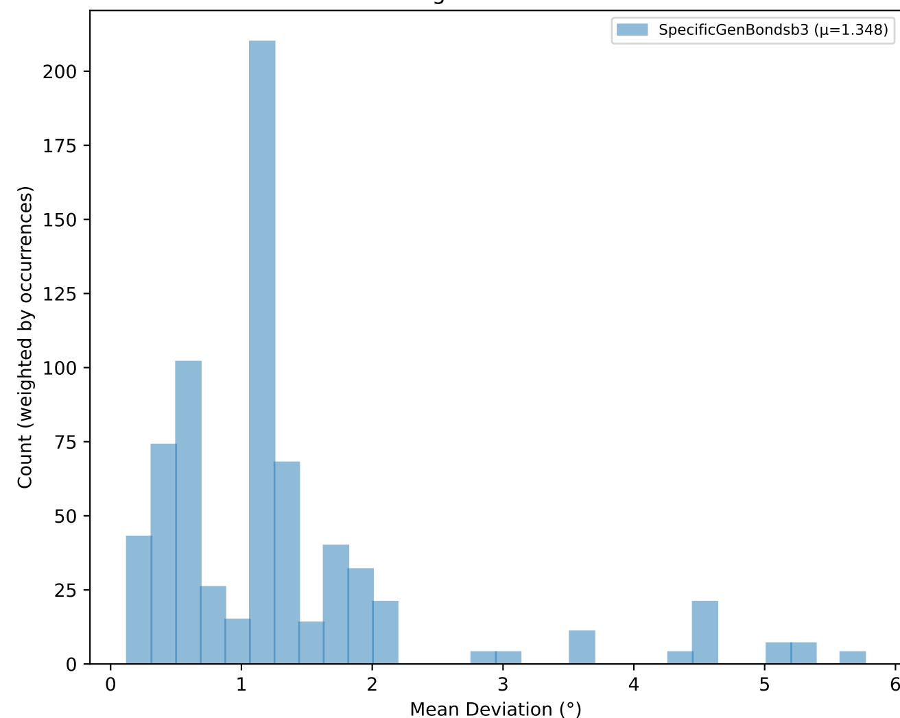
Improper Torsion Deviations
