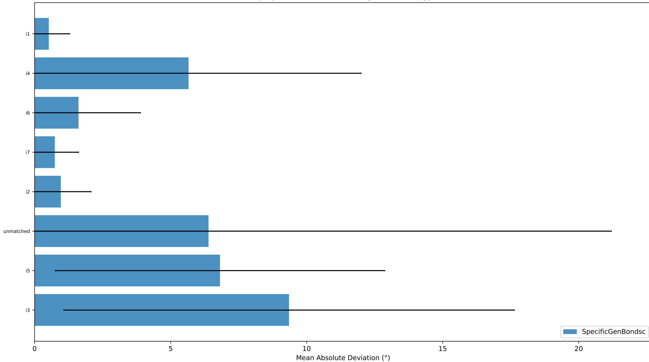
Improper Torsion Deviations by Parameter Type
