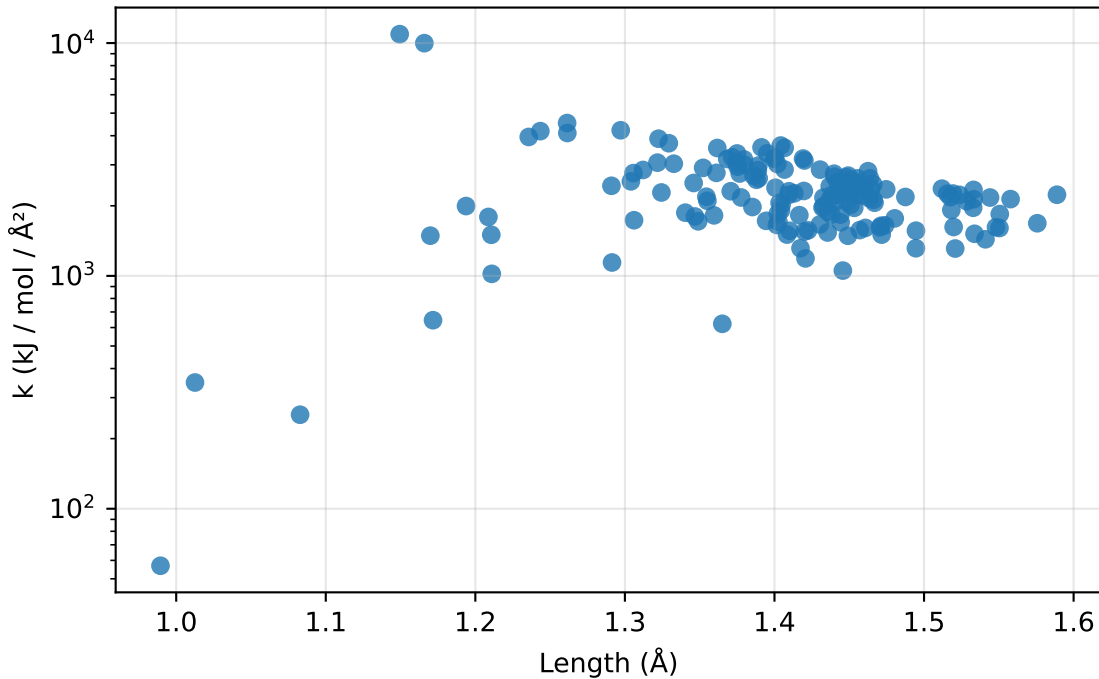
Bonds: k vs length for C-N (160 params)
