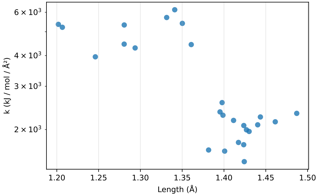
Bonds: k vs length for N-O (26 params)
